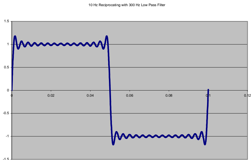
10 Hz Reciprocating Frequency Square Wave with 300 Hz Low Pass Filter
