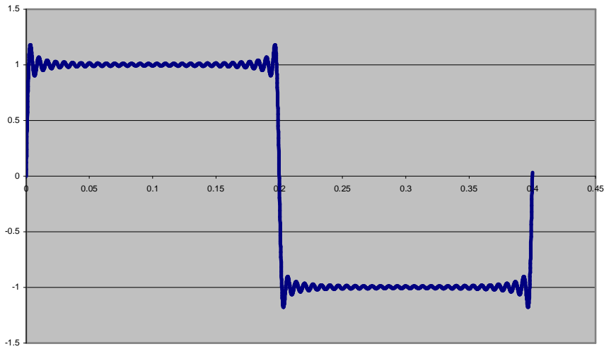
2.5 Hz Reciprocating with 150 Hz Low Pass Filter
