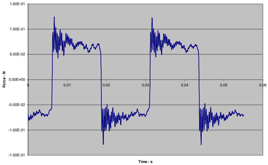
High Speed Force Signal Plotted in Time Domain
