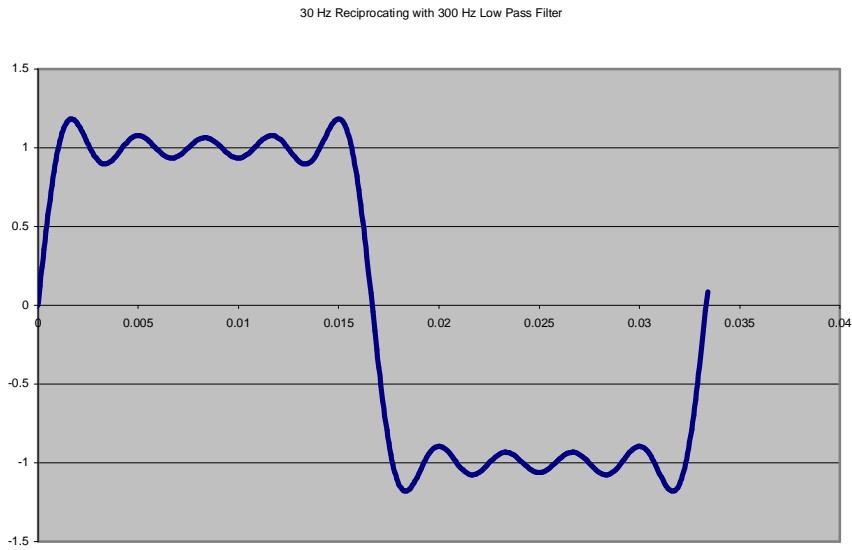
30 Hz Reciprocating Frequency Square Wave with 300 Hz Low Pass Filter High frequency component reduced and signal attenuated
