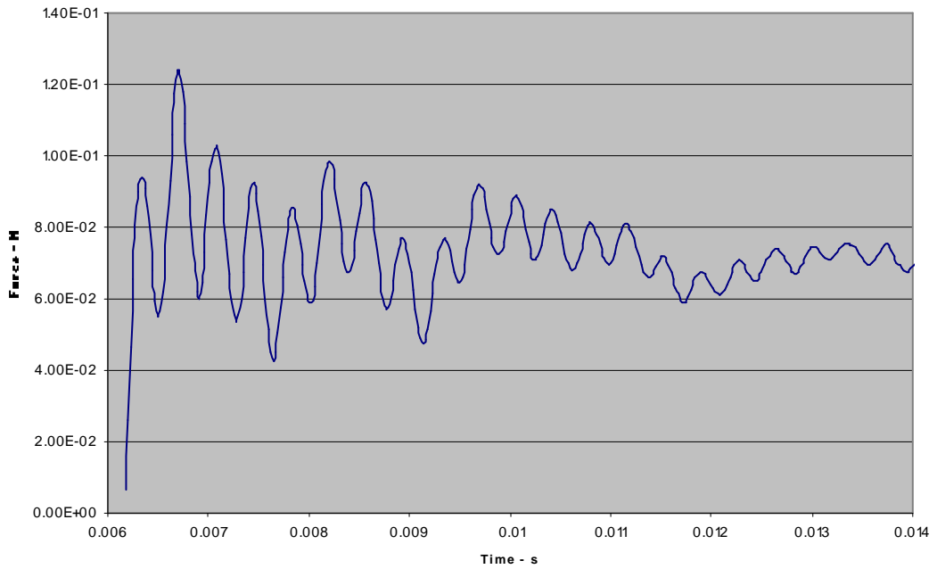
Force Signal Detail – Stroke Beginning
