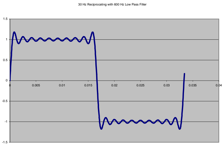
30 Hz Reciprocating Frequency with 600 Hz Low Pass Filter
