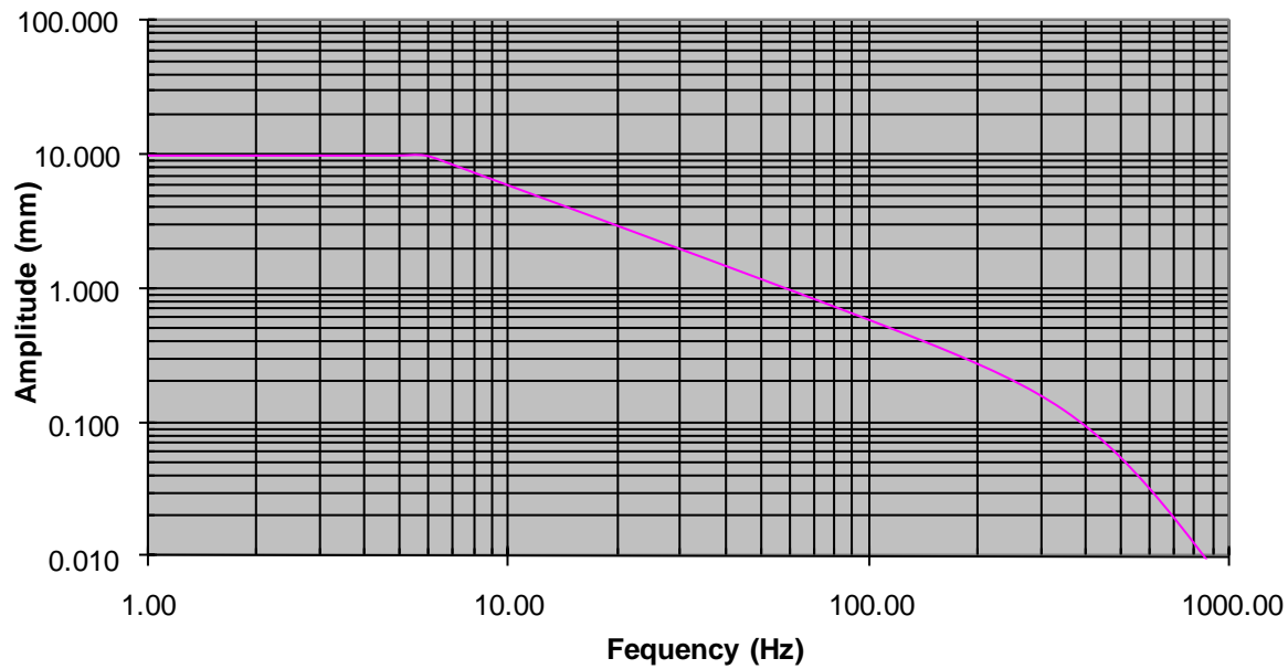
Typical Performance Curve Servo Hydraulic Actuator
