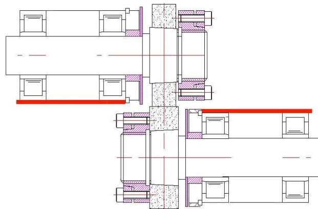
Overhung with Opposed Shafts
