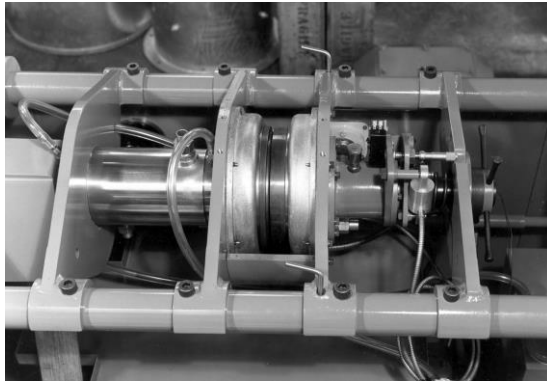
High-pressure seal test machine
