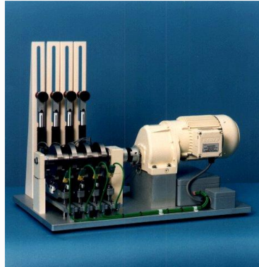
TE 57 Pressurized Lubricity Tester
