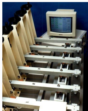
TE 88 Reciprocating Pin on Plate Machine
